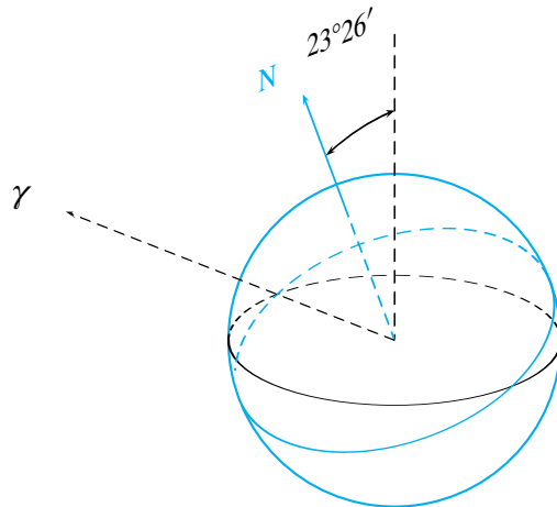
FIGURE 9 – Point gamma
